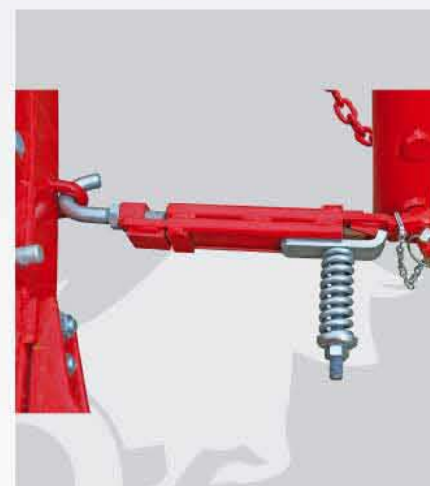
Balansna letva Safety release device
