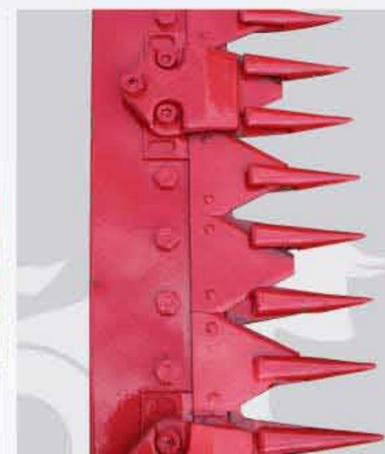
Segment reznog aparata Section of the cutter bar
